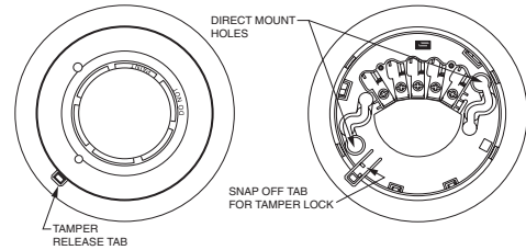
Figure 2: Tamper-Resistant Feature
