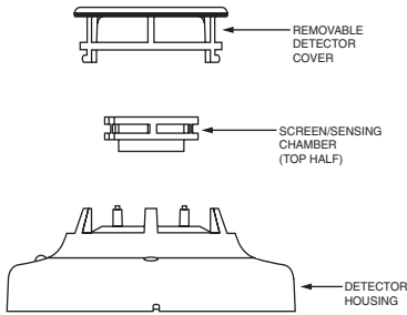
Figure 5: Removing/Replacing Screen/Sensing Chamber
