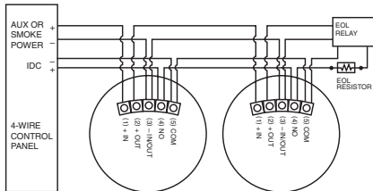
Figure 3: Wiring Diagram
